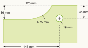
Resaque Pivote Superior
