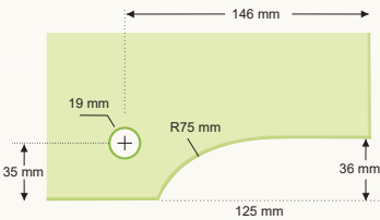
Resaque Chapa
